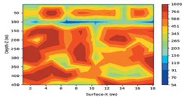
Earth Depth Profile
