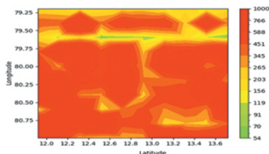
Earth Lat-Long Profile
