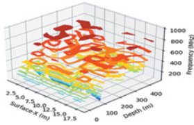
Earth Depth Profile
